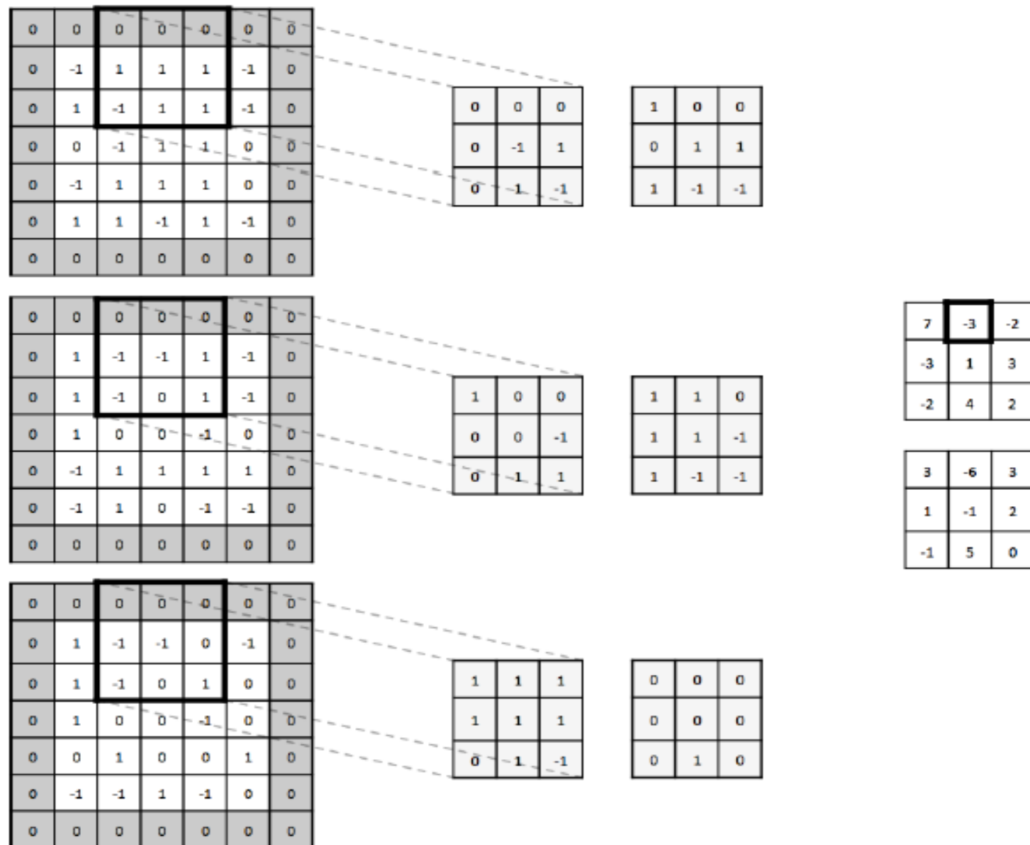
Figure 5-12. Using the same setup as Figure 5-11, we generate the next value in the first length slice of the output volume
